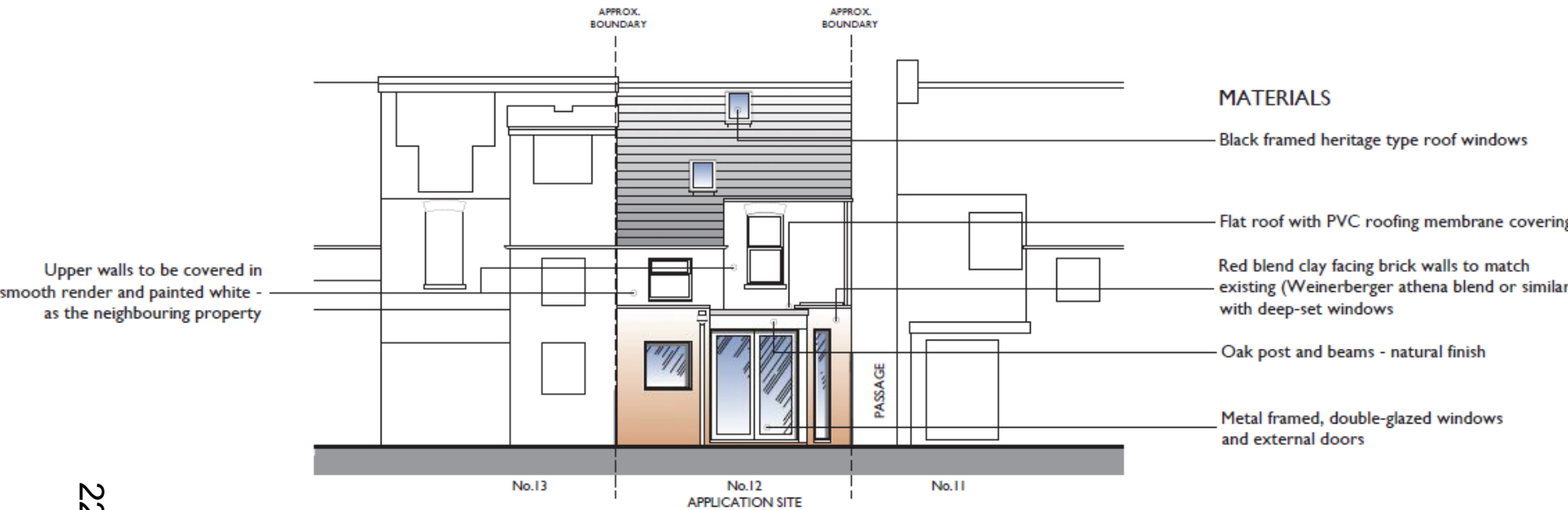
EAST (GARDEN) ELEVATION
